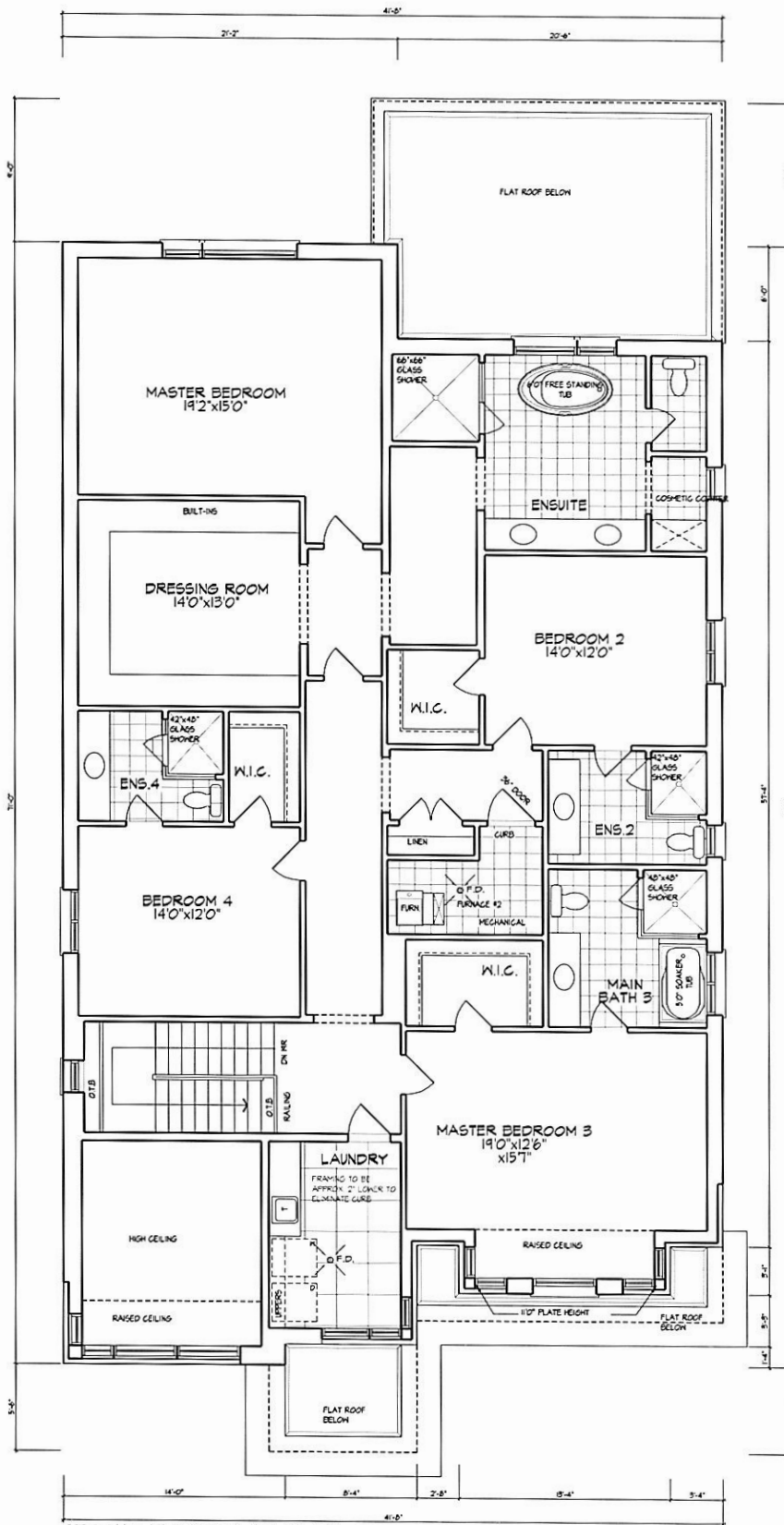
SECOND FLOOR PLAN, EL. 'B' 2560 sq. ft. GROSS FLOOR AREA 2711 sq. ft. DECK/OPEN AREAS 151 sq. ft. NET AREA 2560 sq. ft.
