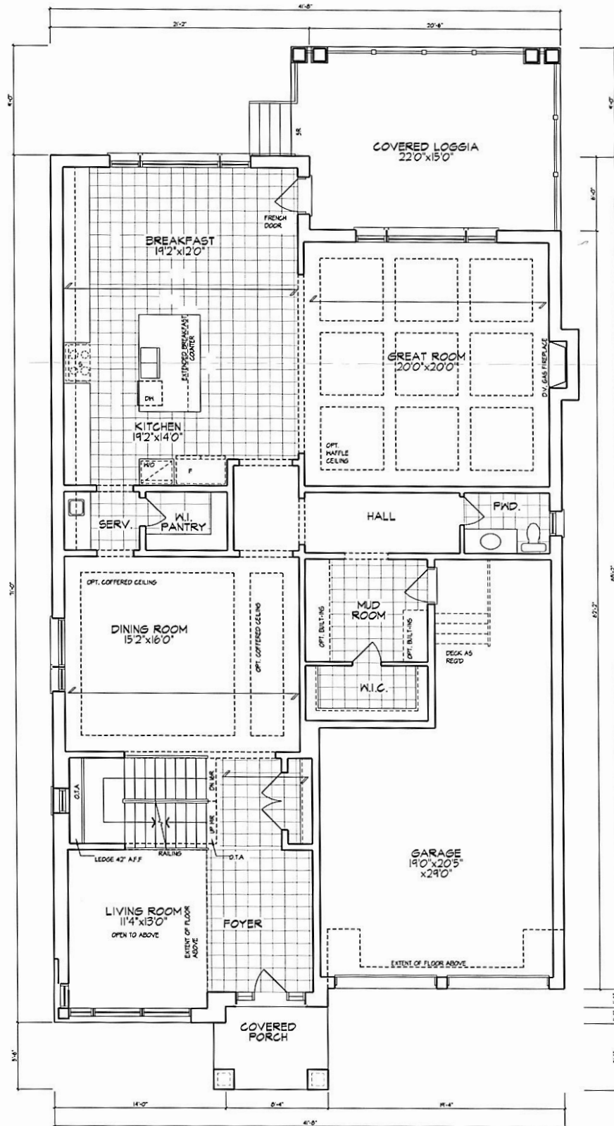
GROUND FLOOR PLAN, EL. 'B' 2221 sq ft COVERAGE W/O PORCH 2178 sq ft COVERAGE W/ PORCH 3049 sq ft (INCLUDES COVERED LOGGIA)
